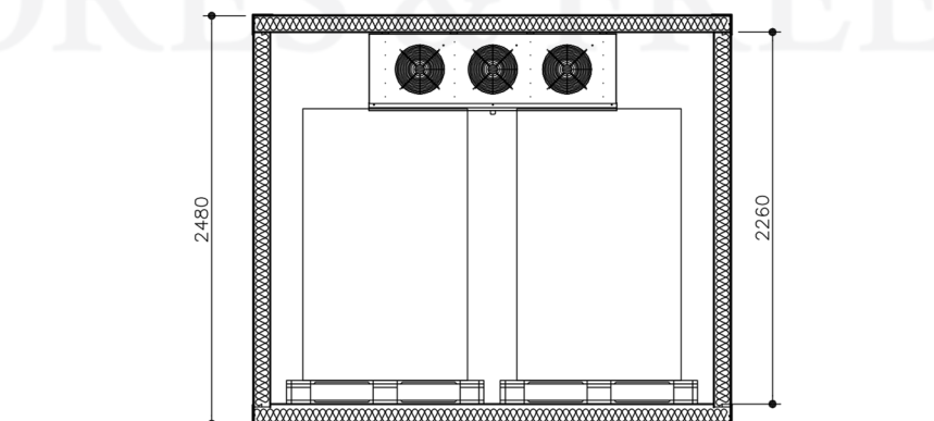
section
