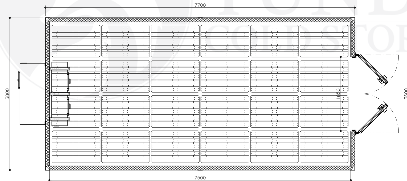
plan
