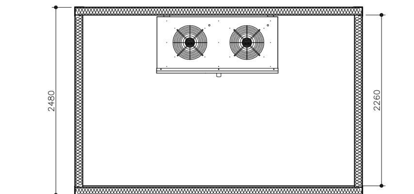
section
