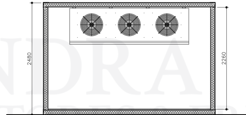
section
